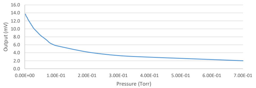
VGT-1504 Thermocouple Gauge (S/N 5078) Calibration Curve - Full Measurement Range
