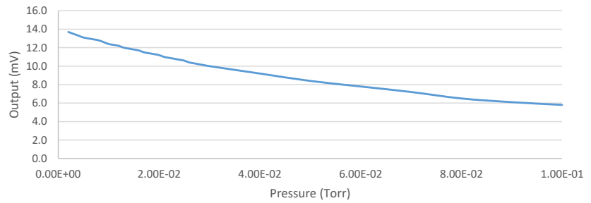
VGT-1504 Thermocouple Gauge (S/N 5078) Calibration Curve - Partial Measurement Range
